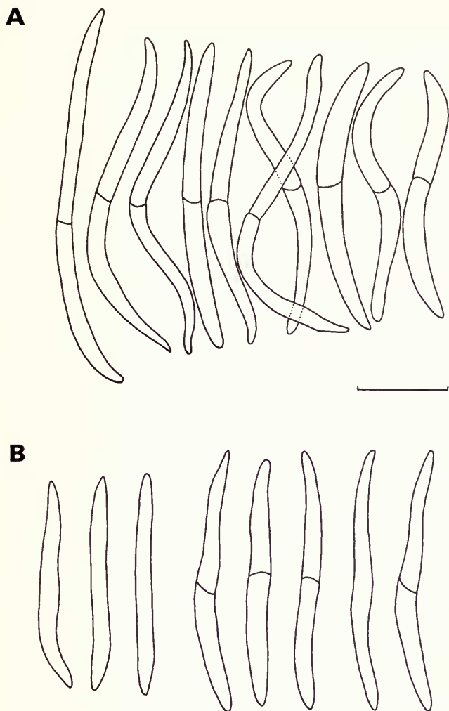
Fig. 6 Ascospore outlines (A) Leptorhaphis contorta Degelius (Degelius-holotype); (B) Leptorhaphis deformis Norman (O-holotype); scale = 10 \mu\text{m} .
